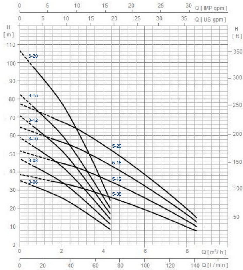
HYDRAULIC PERFORMANCE TABLE
